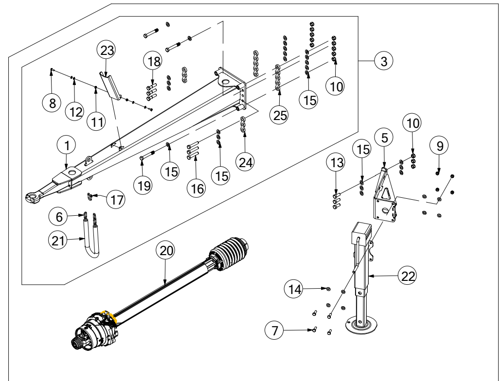
DRAWBAR LOW / HIGH
