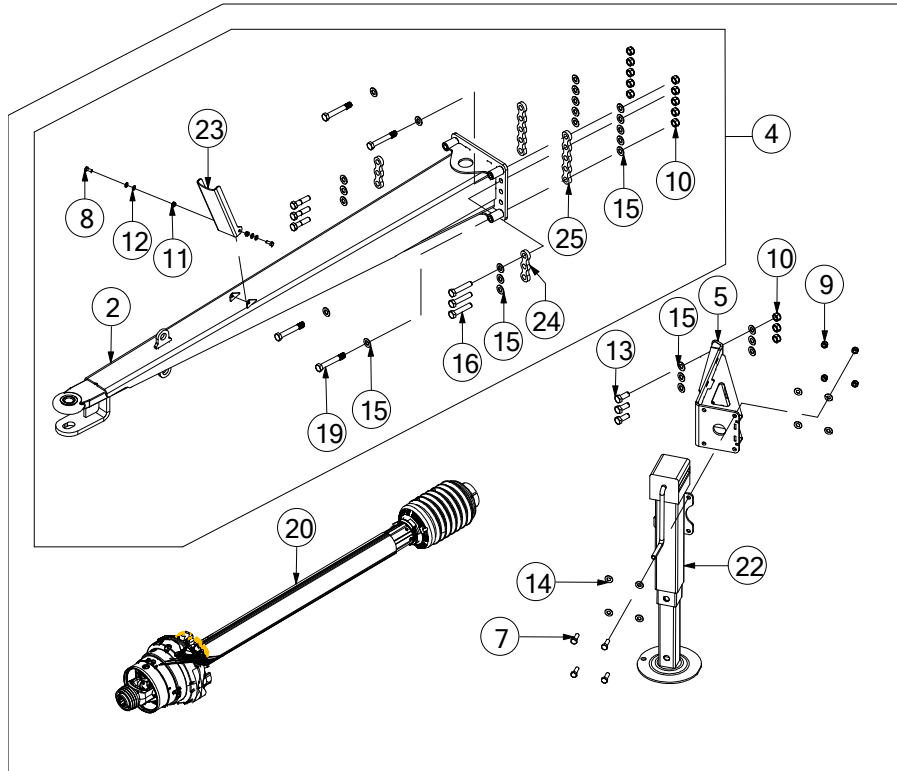
DRAWBAR CLEVIS TYPE
